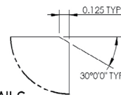
DETAIL C SCALE 1 : 1
