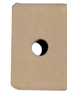
Hydrant Block 5 1 / 2 " x 8" x 1 1 / 2 " Opening 1 3 / 8 "
